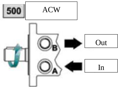
Travel motor rotation direction diagram
